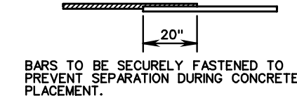
TYPICAL LONGITUDINAL LAP
