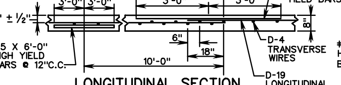
LONGITUDINAL SECTION EXTRA BAR METHOD
