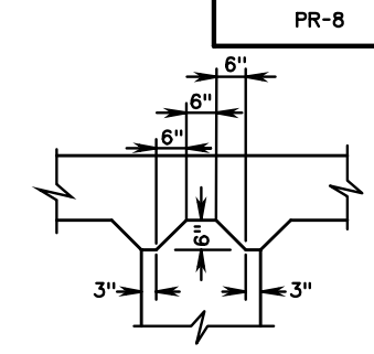
DETAIL A RAISED KEY CONSTRUCTION JOINT
