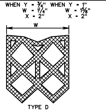
SEALANTS FOR TRANSVERSE EXPANSION JOINTS
