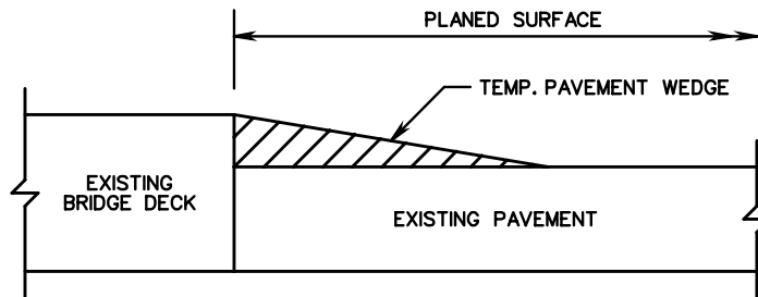
WEDGE DETAIL
