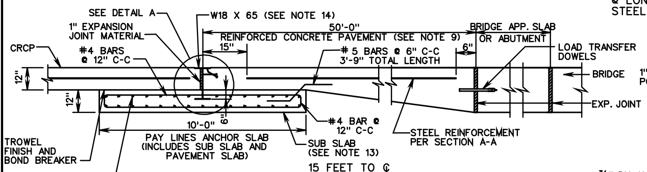
SECTION F-F ANCHOR SLAB TYPE II (SEE NOTE 11)
