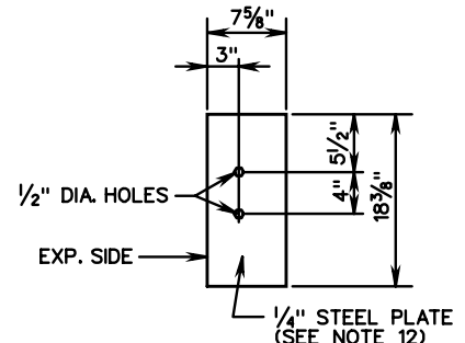
ANCHOR SLAB TYPE II END PLATE DETAIL
