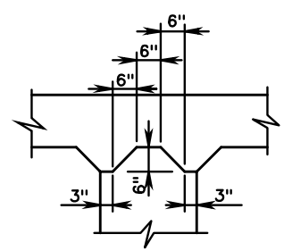
DETAIL A RAISED KEY CONSTRUCTION JOINT
