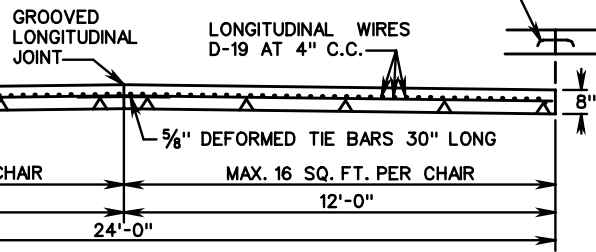
TRANSVERSE SECTION
