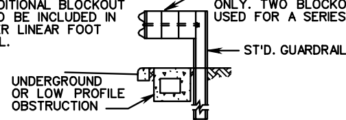
SECTION D-D DETAIL OF MULTIPLE BLOCK-OUT TO AVOID UNDERGROUND OR LOW PROFILE OBSTRUCTION
