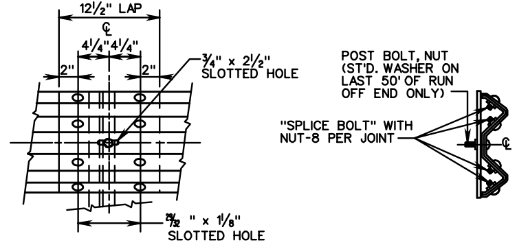
LAP IN DIRECTION OF TRAFFIC DETAIL OF SPLICE JOINT
