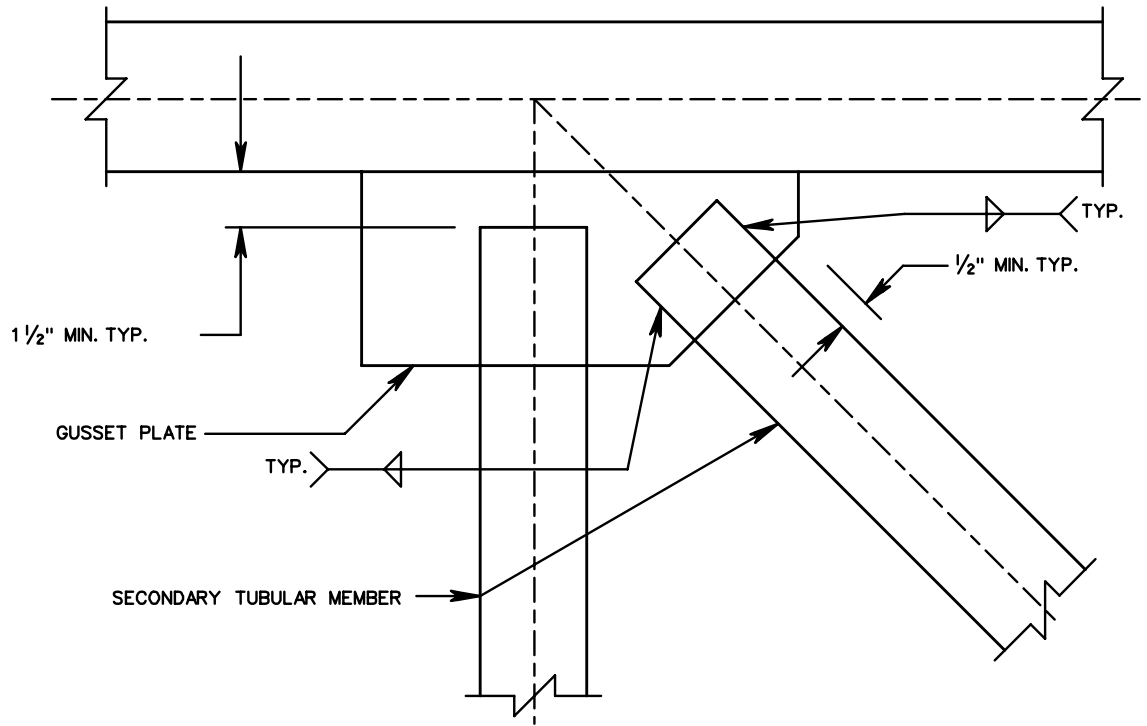
TYPICAL GUSSET PLATE CONNECTION
