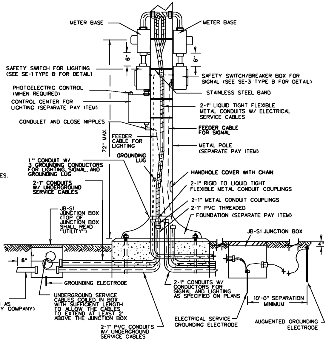
TYPE B (UNDERGROUND SERVICE) METAL POLE
