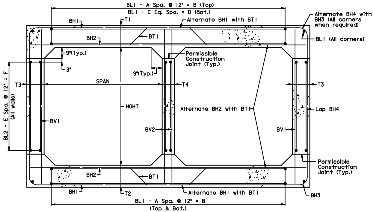
TYPICAL SECTION
