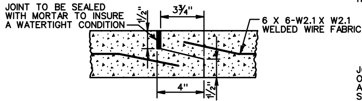
PRECAST CONCRETE VEE DITCH
