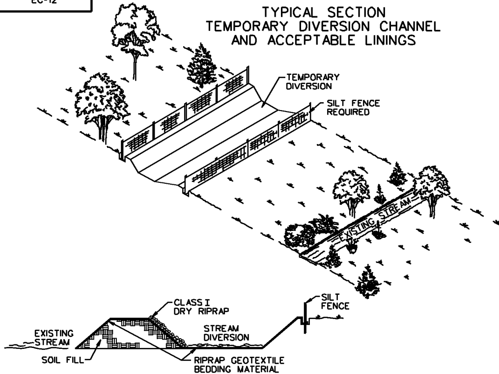
DAM DETAIL
