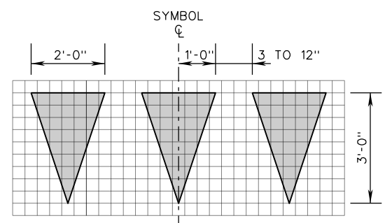
YIELD TRIANGLE LINE LAYOUT (2' x 3' TRIANGLES)
