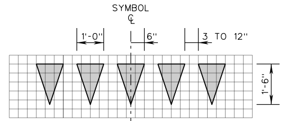
YIELD TRIANGLE LINE LAYOUT (1' x 1.5' TRIANGLES)
