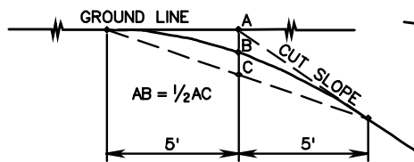
DETAILS OF ROUNDING TOPS OF CUT SLOPES
