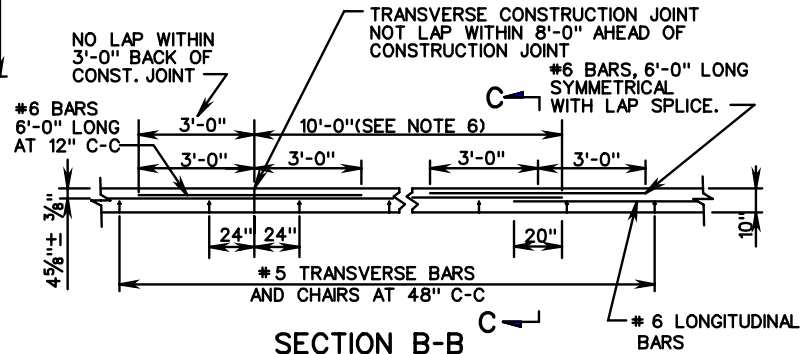
SECTION B-B EXTRA BAR METHOD
