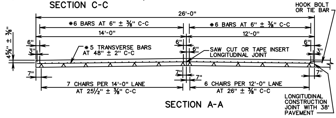
TYPICAL LONGITUDINAL LAP
