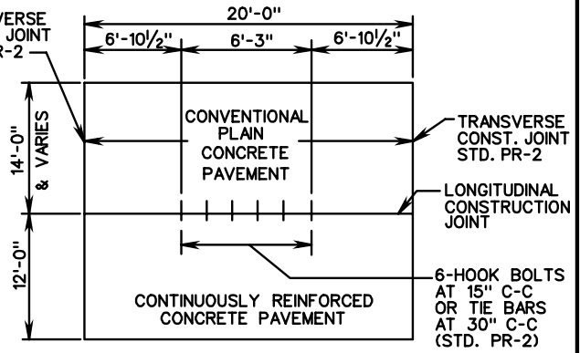
PLAN-RAMP & MAIN LINE CONNECTION
