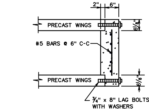
END WALL DETAIL
