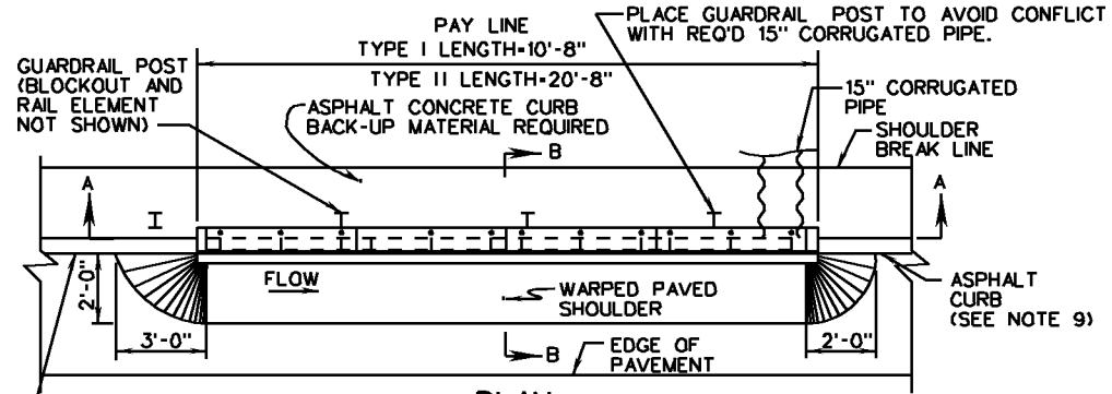
PLAN (ROADWAY LOCATION)
