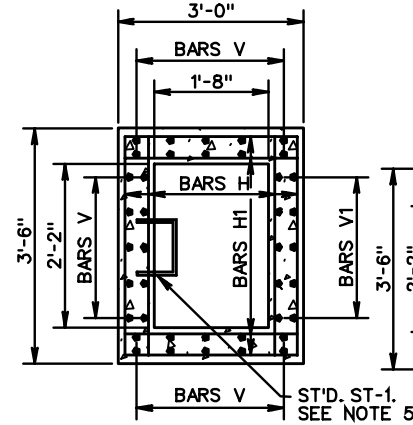
SECTION C-C TYPE I & III
