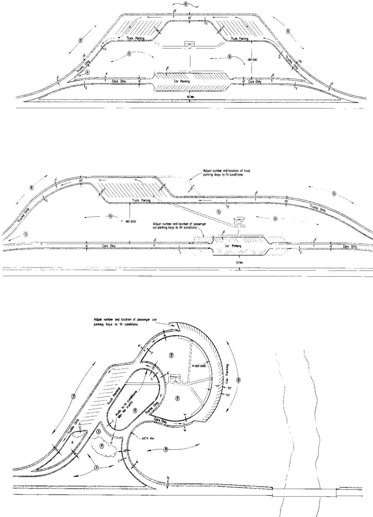
FIGURE C-1-16 EXAMPLES OF SITE LAYOUTS FOR REST AREAS
