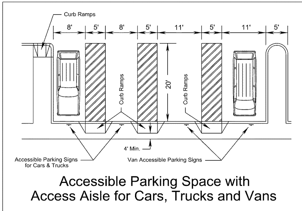
FIGURE C-1-8 ACCESSIBLE PARKING SPACE WITH ACCESS AISLE FOR CARS, TRUCKS AND VANS
