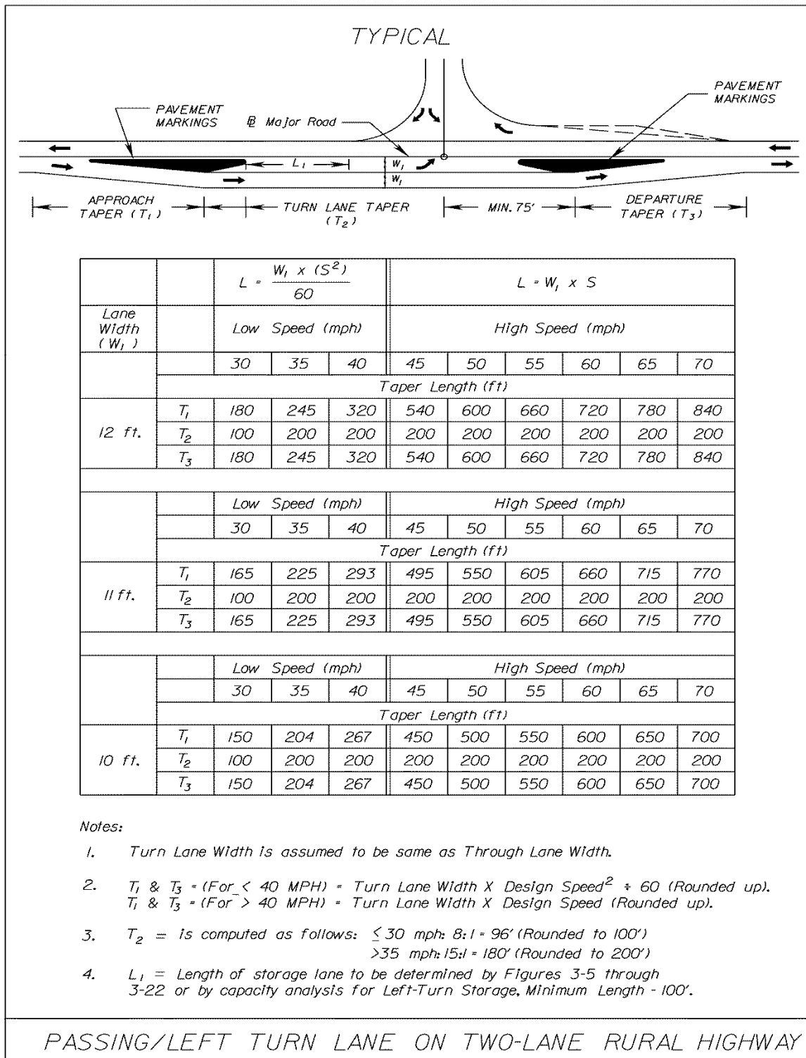
FIGURE 3-4 PASSING/LEFT TURN LANE ON TWO-LANE RURAL HIGHWAY
