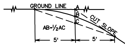
DETAILS OF ROUNDING TOPS OF CUT SLOPES
