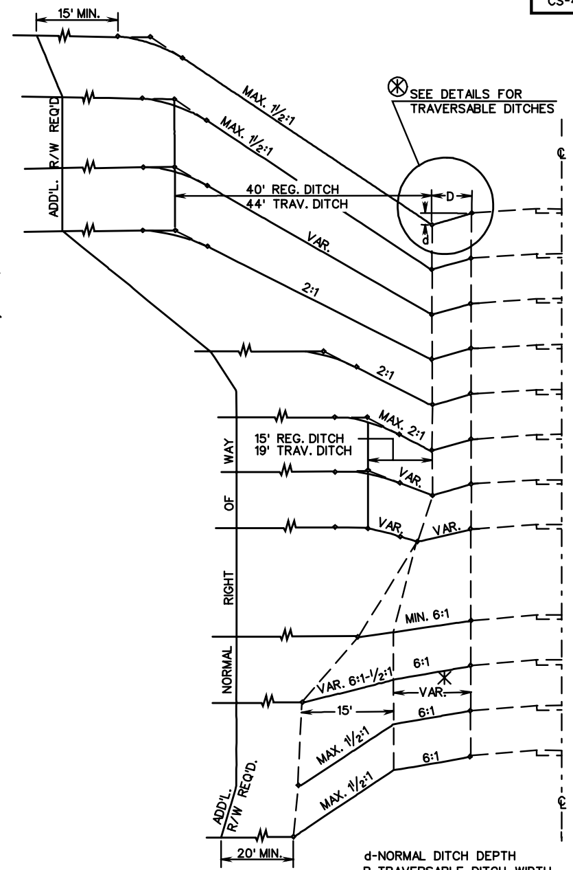
DETAIL SHOWING BERM DITCH IF SHOWN ON PLANS OR REQ'D. BY THE ENGINEER
