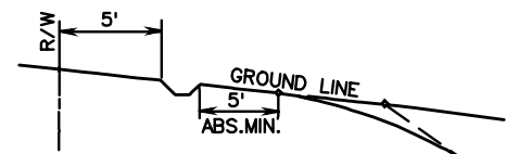
DETAIL SHOWING BERM DITCH IF SHOWN ON PLANS OR REQ'D. BY THE ENGINEER
