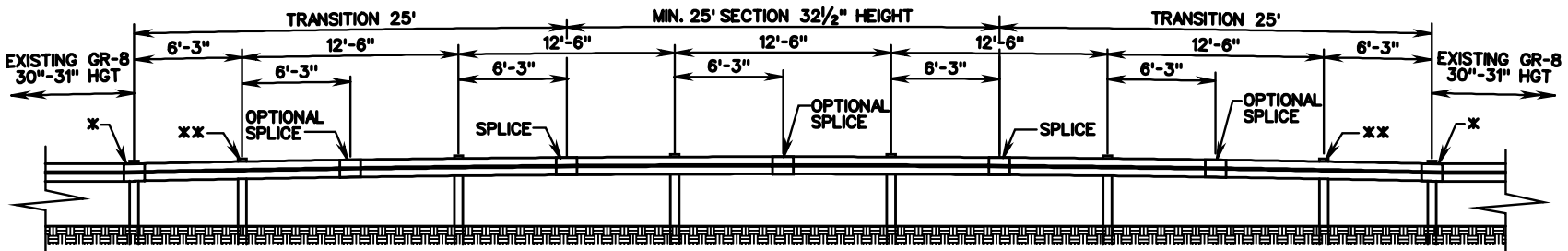
TRANSITION FROM WEAK POST (STANDARD GR-8) TO STRONG POST (STANDARD GR-2) GUARDRAIL
