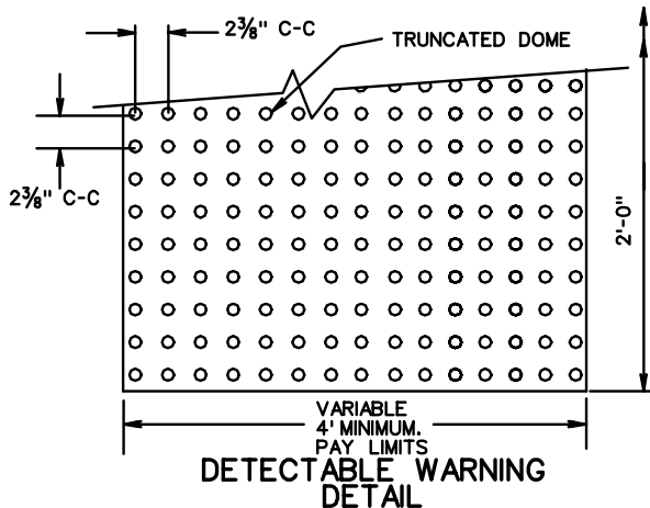
TRUNCATED DOME DETAIL
