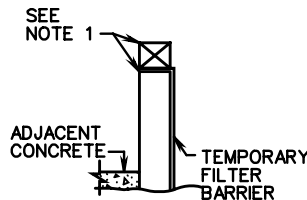
TYPICAL TREATMENT FOR DROP INLET WITHOUT CONCRETE GUTTER
