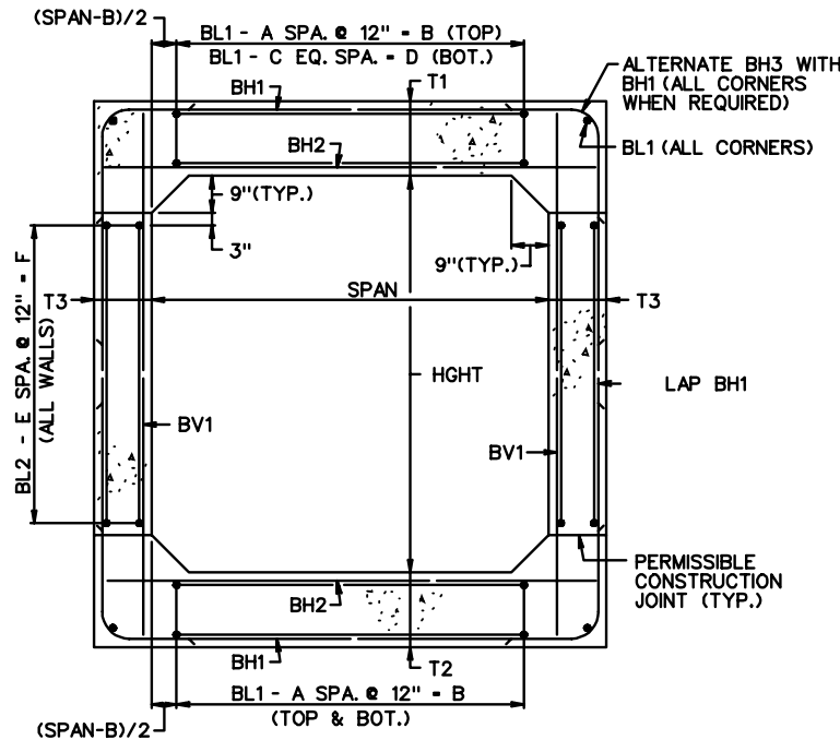
TYPICAL SECTION
