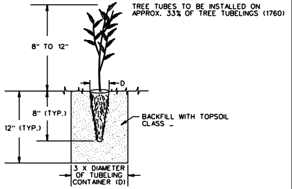
PLANTING TREE TUBELING
