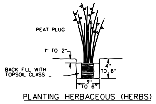
PLANTING HERBACEOUS (HERBS)
