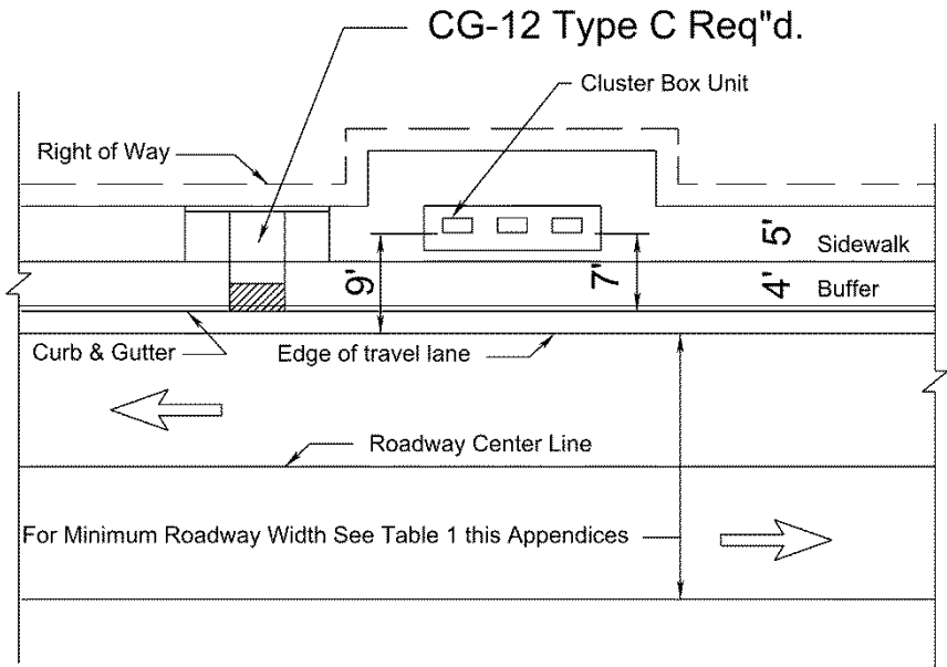
Detail for Cluster Box Unit Without Turnout – Curb & Gutter Typical Section
