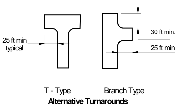
FIGURE 4 – CUL-DE-SAC DETAILS*
