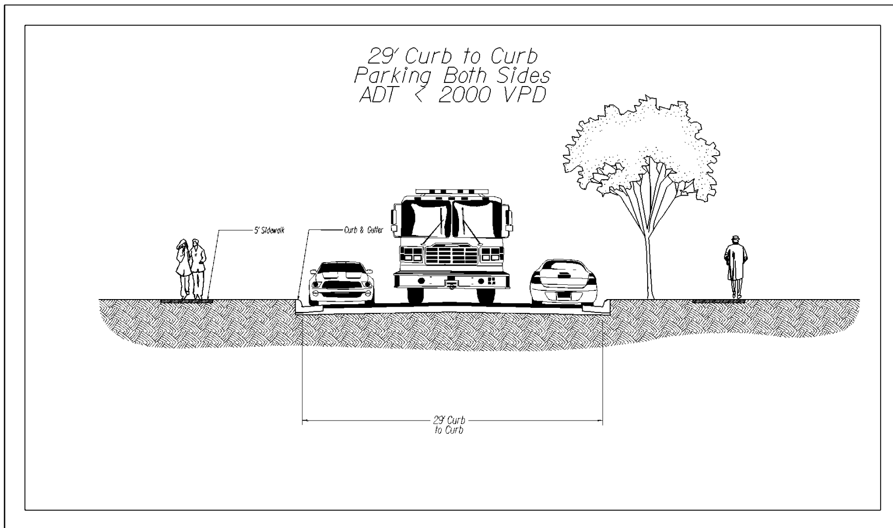
FIGURE 1.4 – 29' CURB TO CURB PARKING ON BOTH SIDES*
