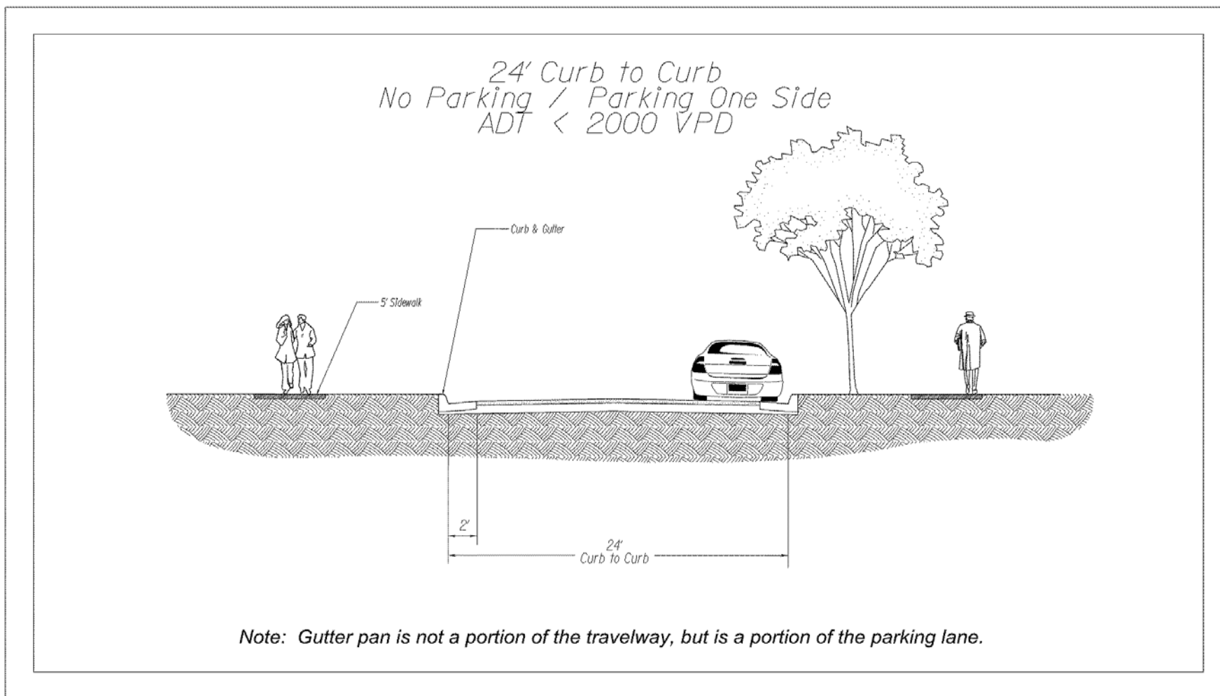
FIGURE 1.1 – 24' CURB TO CURB NO PARKING / PARKING ON ONE SIDE*
