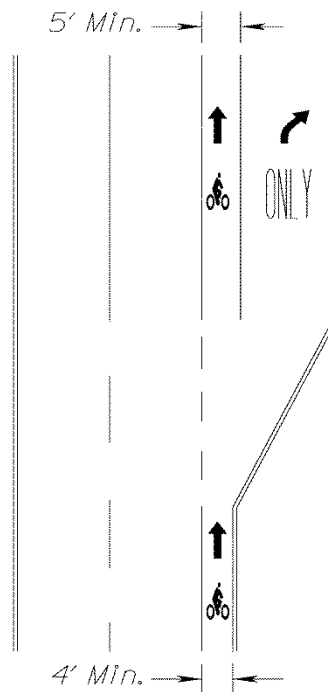
FIGURE A-5-3 RIGHT TURN ONLY LANE
