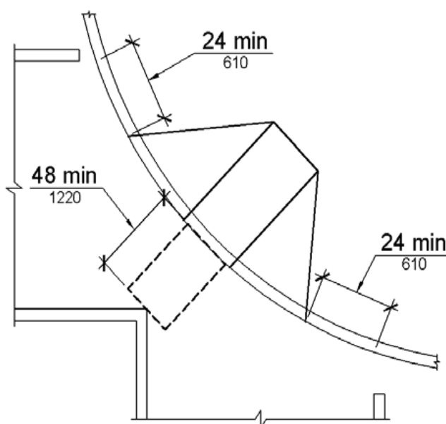
FIGURE A-5-16 DIAGONAL OR CORNER TYPE CURB RAMPS
