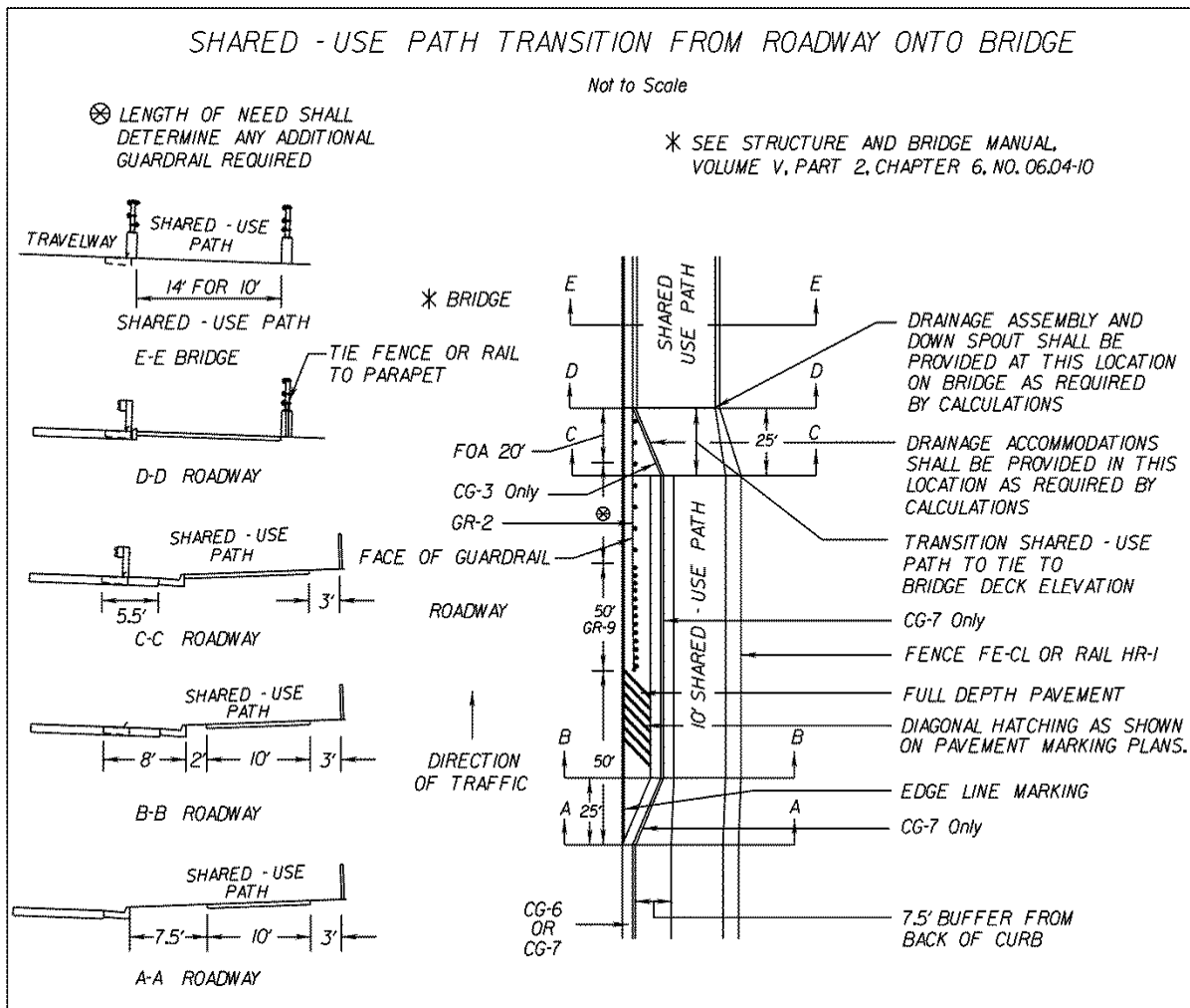
FIGURE A-5-9 SHARED USE PATH TRANSITION FROM ROADWAY ONTO BRIDGE FOR DESIGN SPEEDS >45 MPH*
