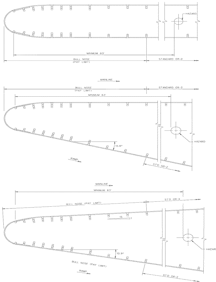
SPECIAL DESIGN BULL NOSE BARRIER
