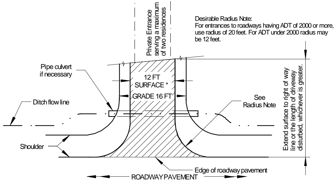
FIGURE 9 – PRIVATE ENTRANCE DETAIL
