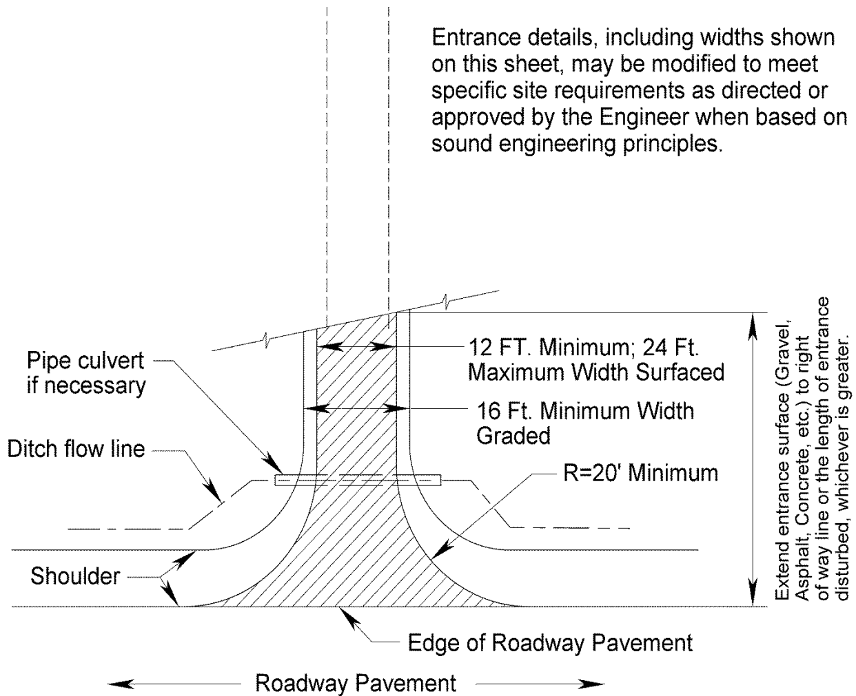
FIGURE 4-1 PRIVATE ENTRANCE AND LOW VOLUME COMMERCIAL ENTRANCE DETAIL*
