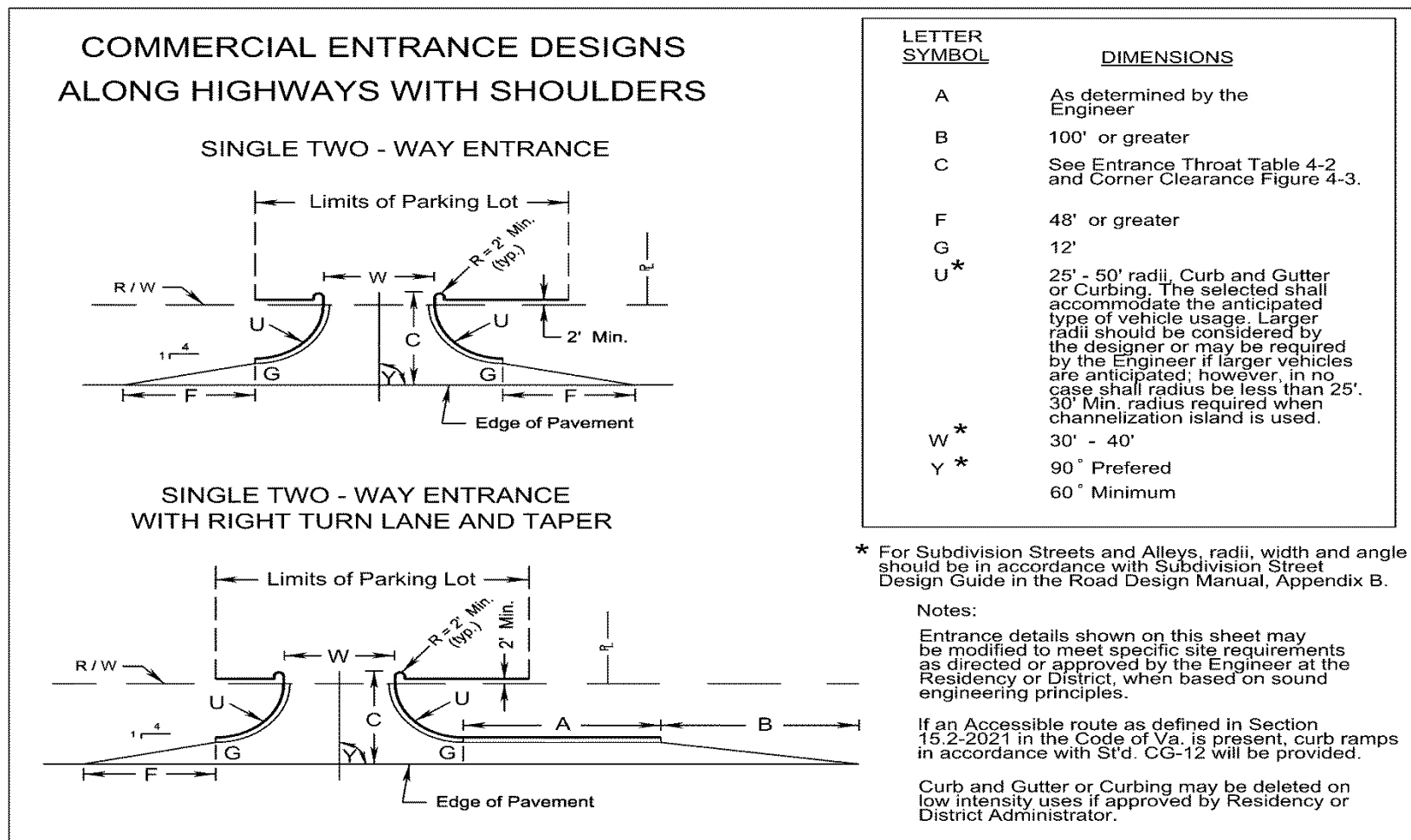
FIGURE 4- 9 COMMERCIAL ENTRANCE DESIGNS ALONG HIGHWAYS WITH SHOULDERS*
