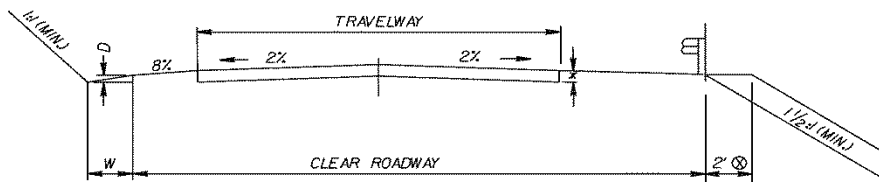
TYPICAL SECTION
