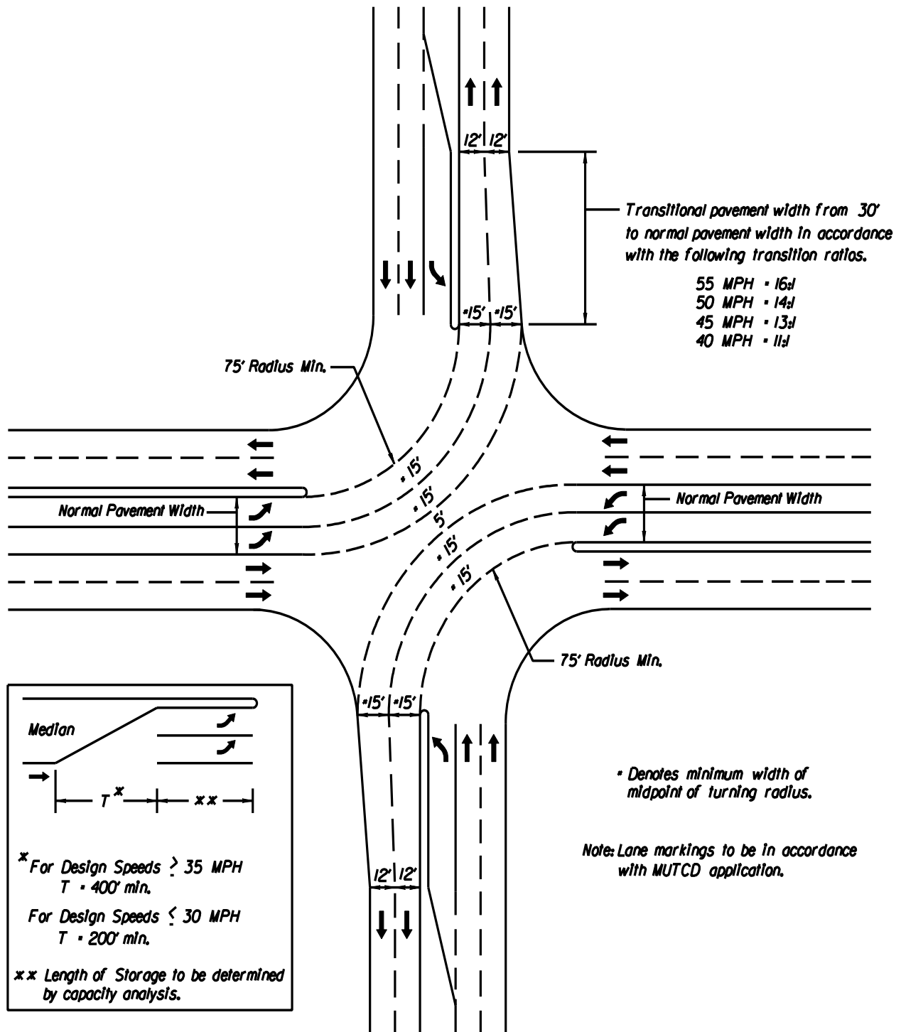
FIGURE 3-23 DOUBLE LEFT-TURN LANES*
