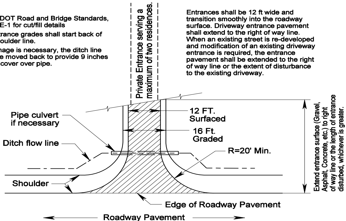
FIGURE 9 – PRIVATE ENTRANCE DETAIL*
