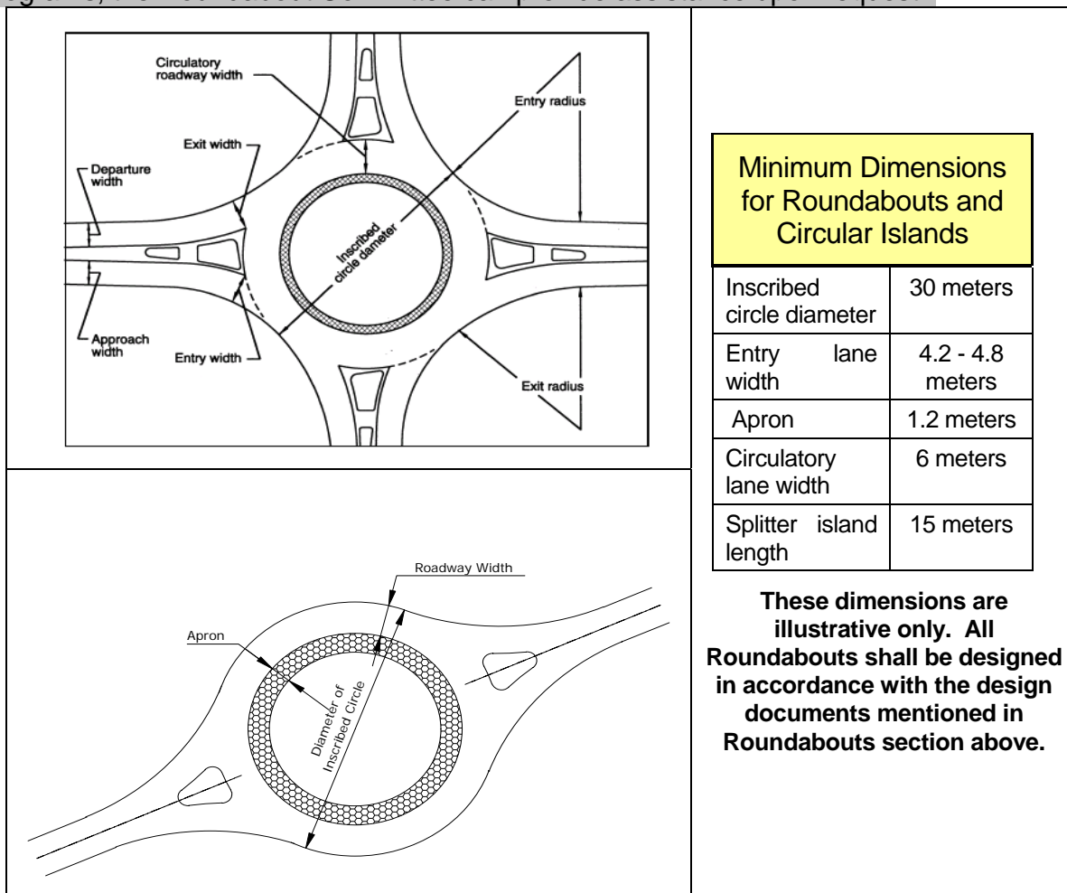
FIGURE C-1-2.2M ROUNDABOUT DETAILS
