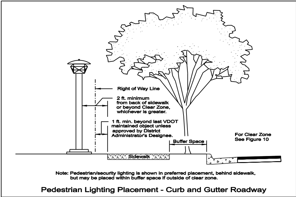
FIGURE 13 – LIGHTING ALONG CURB AND GUTTER SECTIONS*
