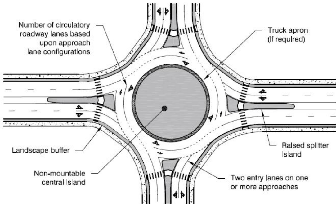
Features of a Typical Multi-Lane Roundabout
