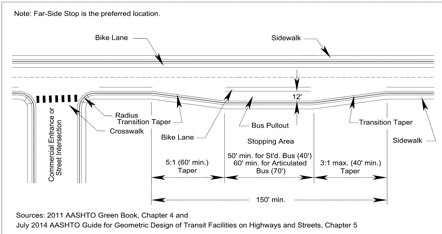
FIGURE 3-29 TYPICAL APPLICATION OF A BUS PULLOUT*
