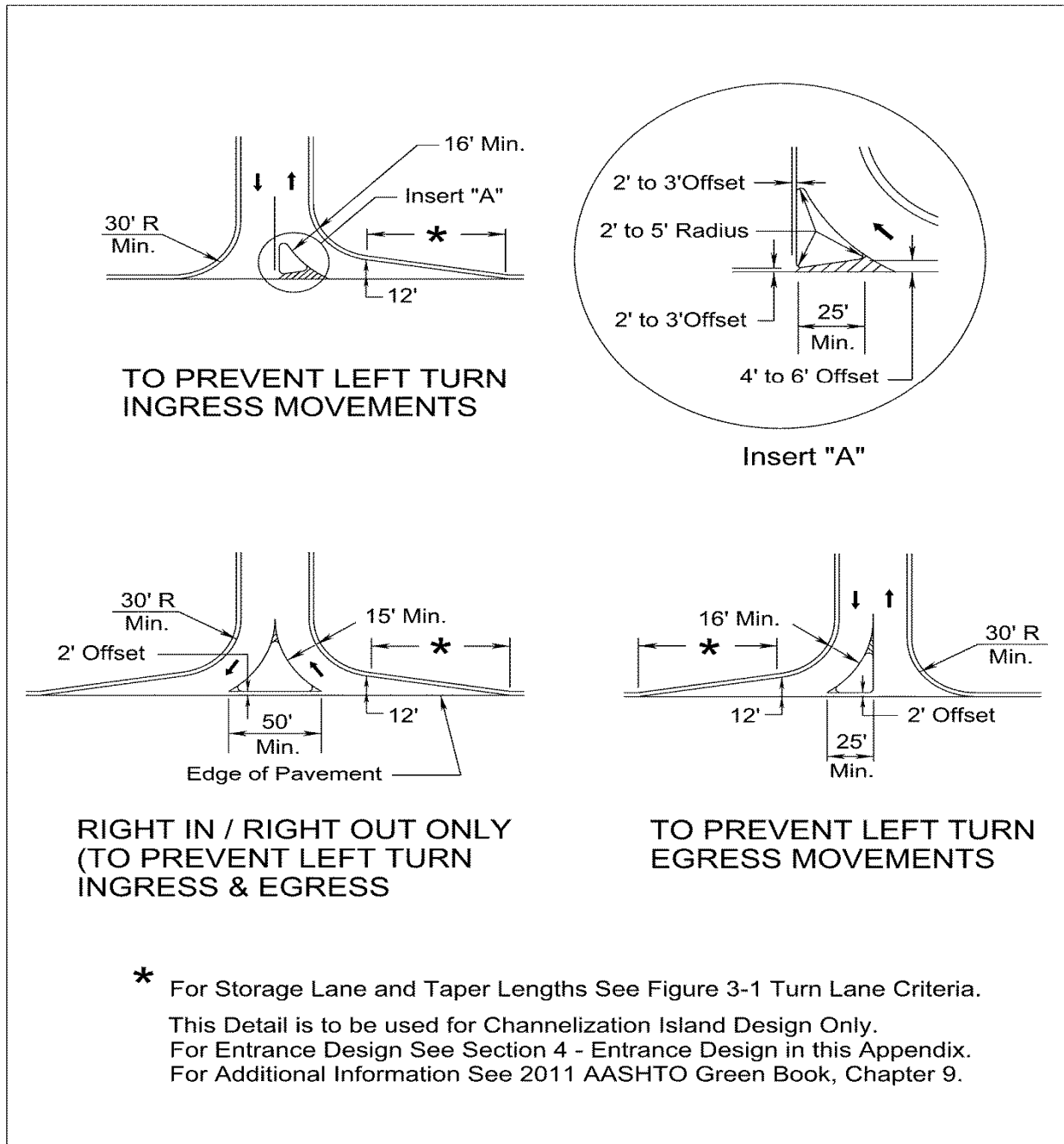
FIGURE 4-4 COMMERCIAL ENTRANCE CHANNELIZATION ISLAND OPTIONS
