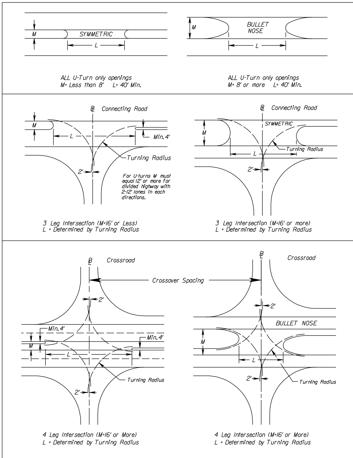
FIGURE 2-13 CROSSOVERS WITH AND WITHOUT CONNECTIONS
