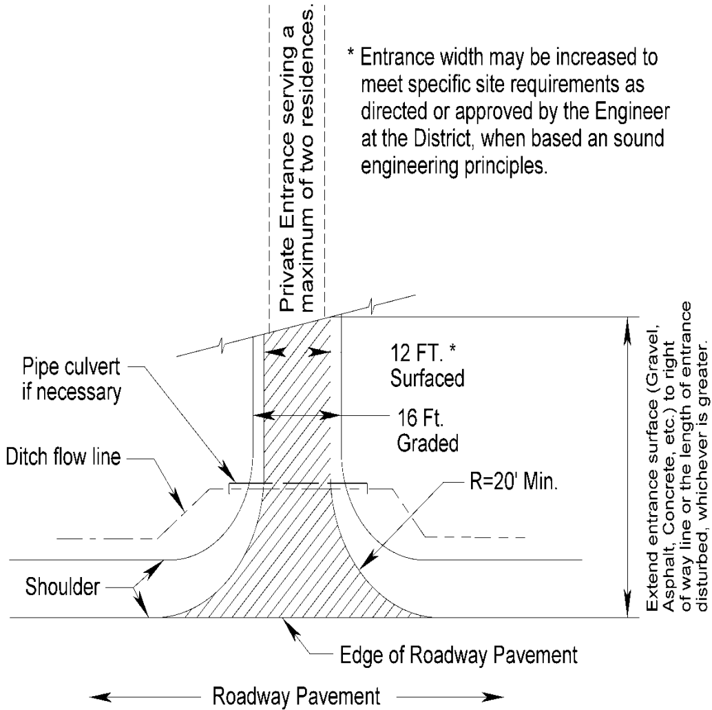
FIGURE 4-1 PRIVATE ENTRANCE AND LOW VOLUME COMMERCIAL ENTRANCE DETAIL*
