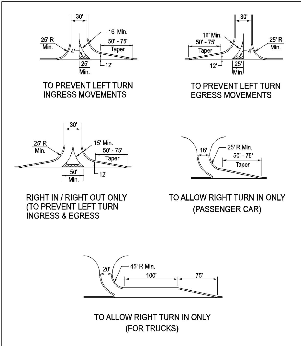
FIGURE 4-5 COMMERCIAL ENTRANCE CHANNELIZATION ISLAND OPTIONS
