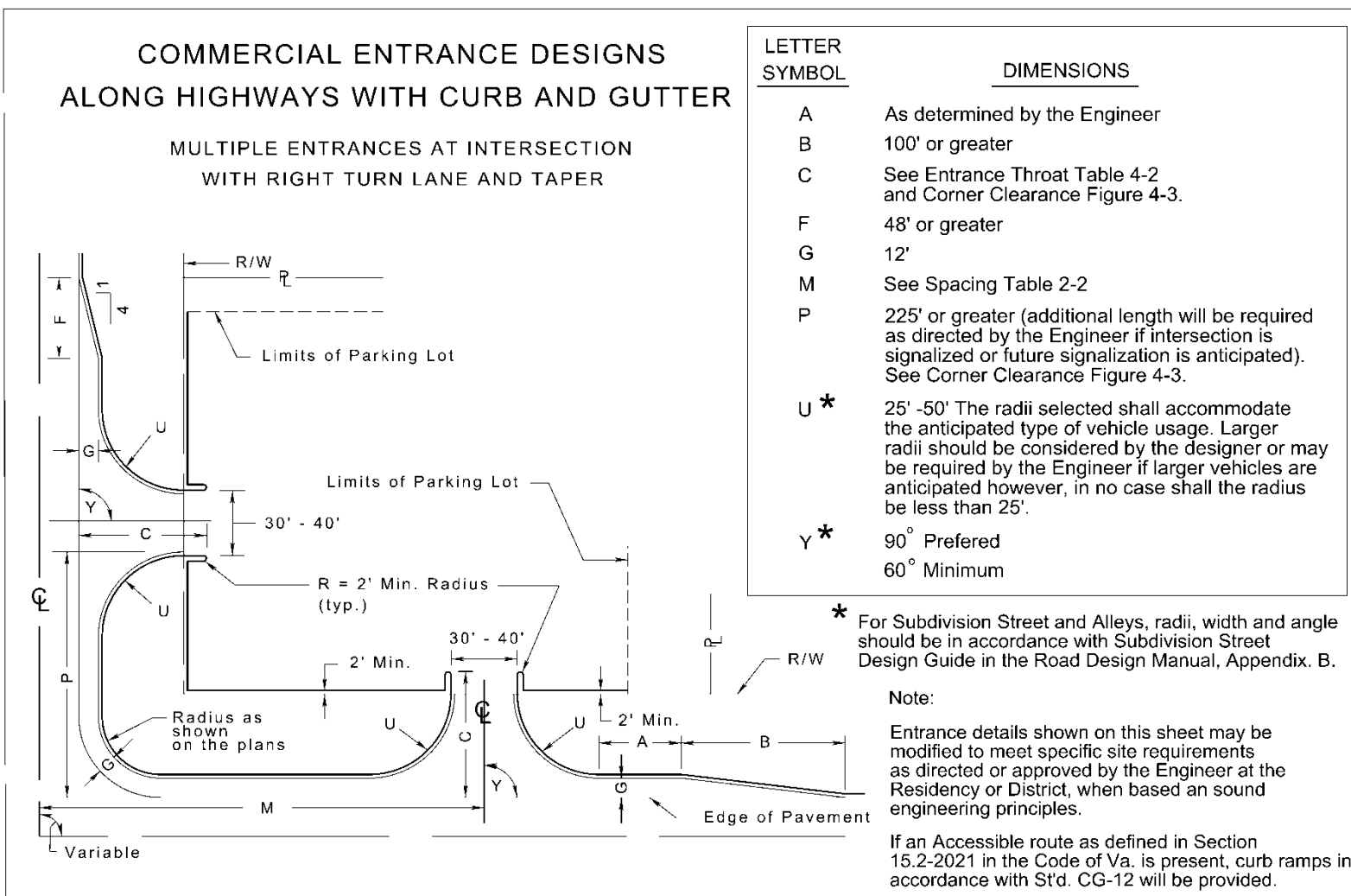
FIGURE 4-13 COMMERCIAL ENTRANCE DESIGNS ALONG HIGHWAYS WITH CURB & GUTTER AT INTERSECTION
