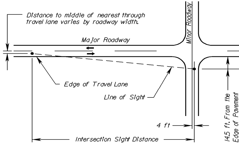
Left Sight Distance Triangle
