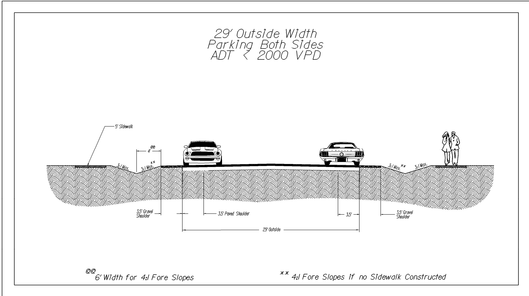
FIGURE 1.6 – 29' OUTSIDE WIDTH PARKING ON BOTH SIDES*
