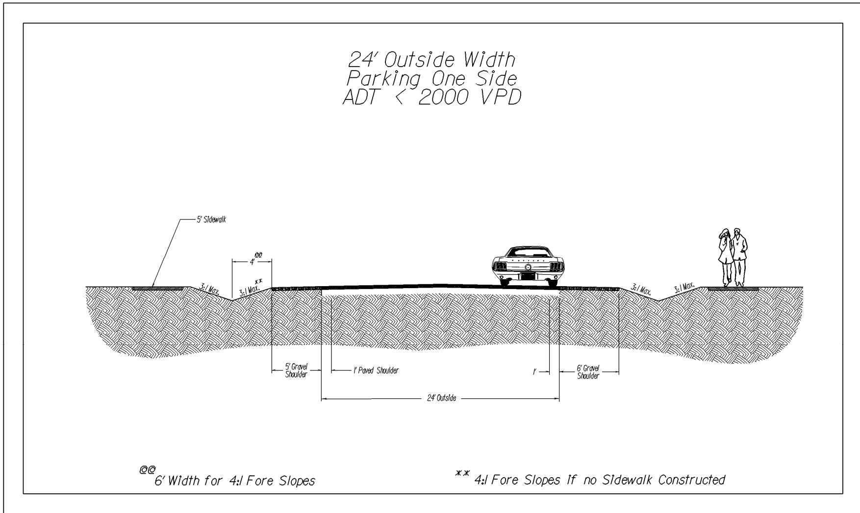
FIGURE 1.5 – 24' OUTSIDE WIDTH PARKING ONE SIDE*
