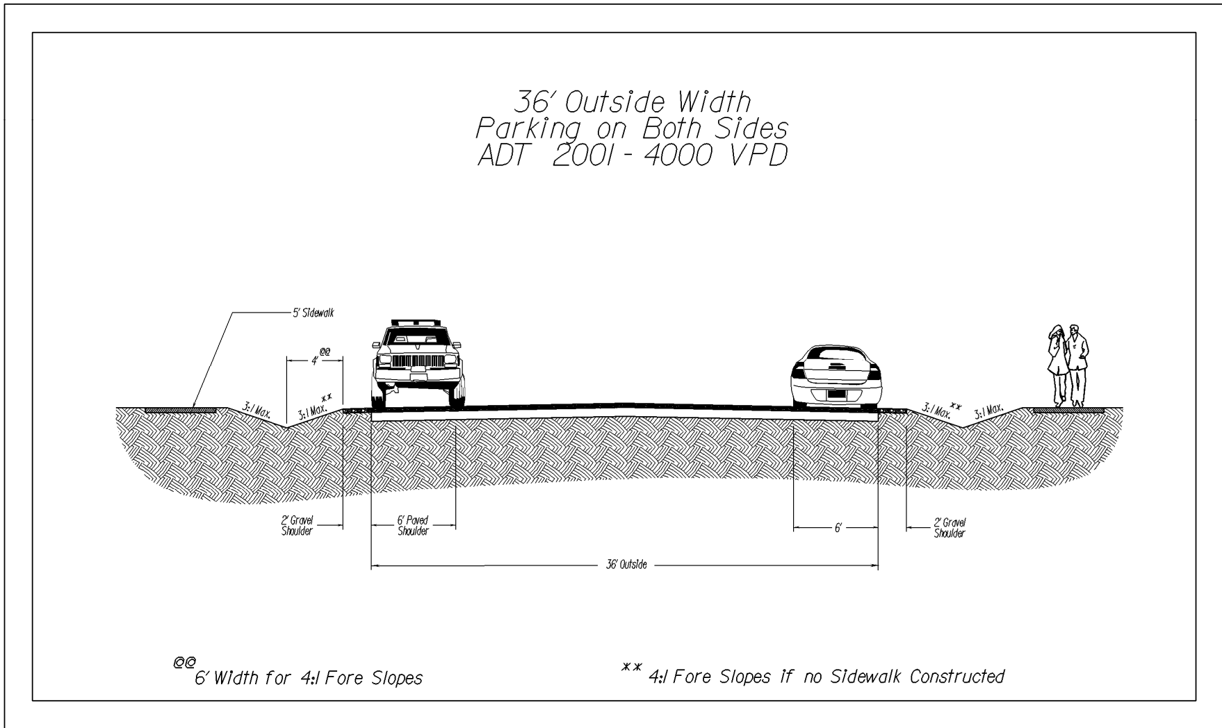
FIGURE 1.7 – 36' OUTSIDE WIDTH PARKING ON BOTH SIDES*
