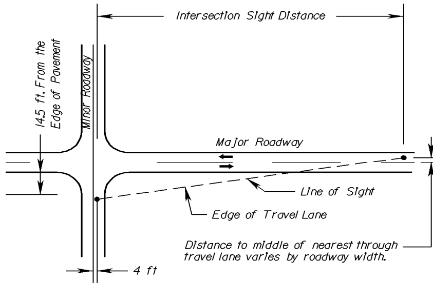
Right Sight Distance Triangle
