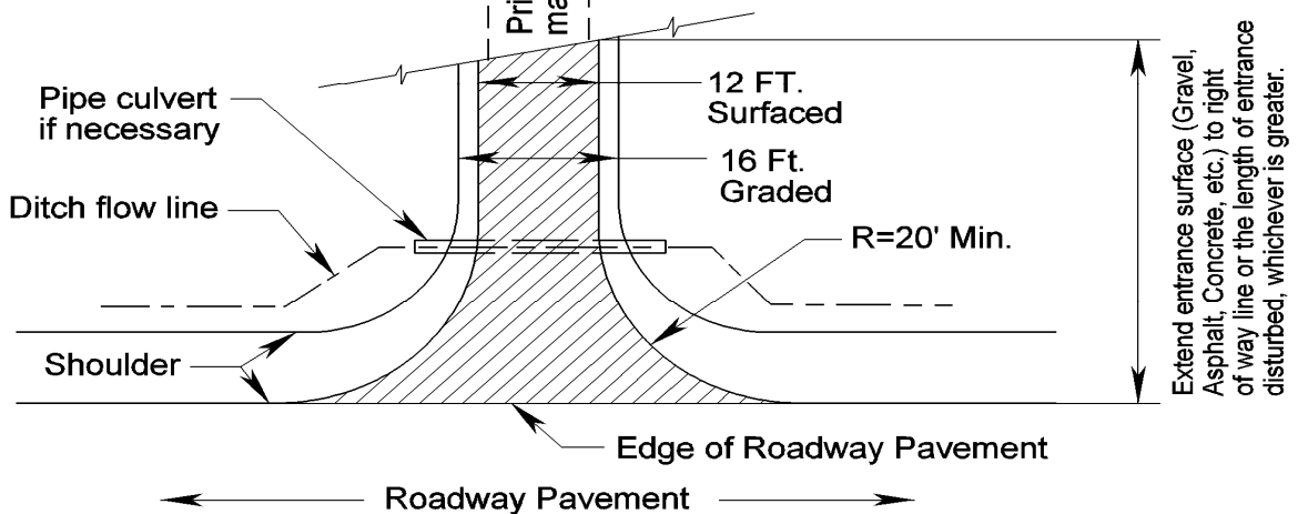
FIGURE 9 – PRIVATE ENTRANCE DETAIL *
