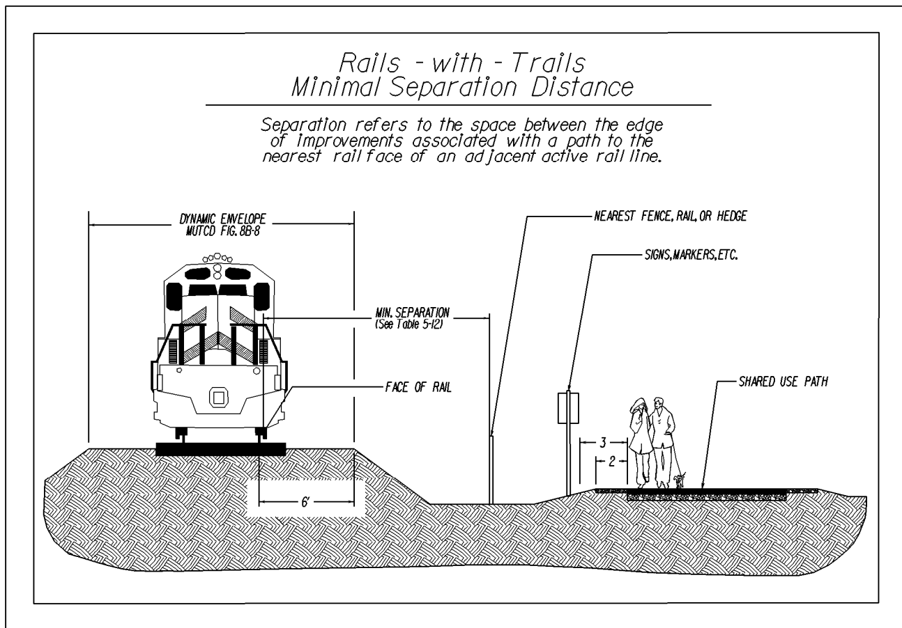
FIGURE A- 5-11 SEPARATION BETWEEN ACTIVE RAIL LINES AND PATHS (RWT)
