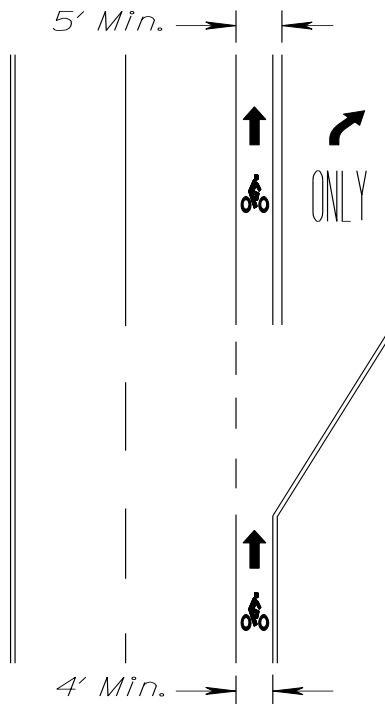
FIGURE A-5-3 RIGHT TURN ONLY LANE*
