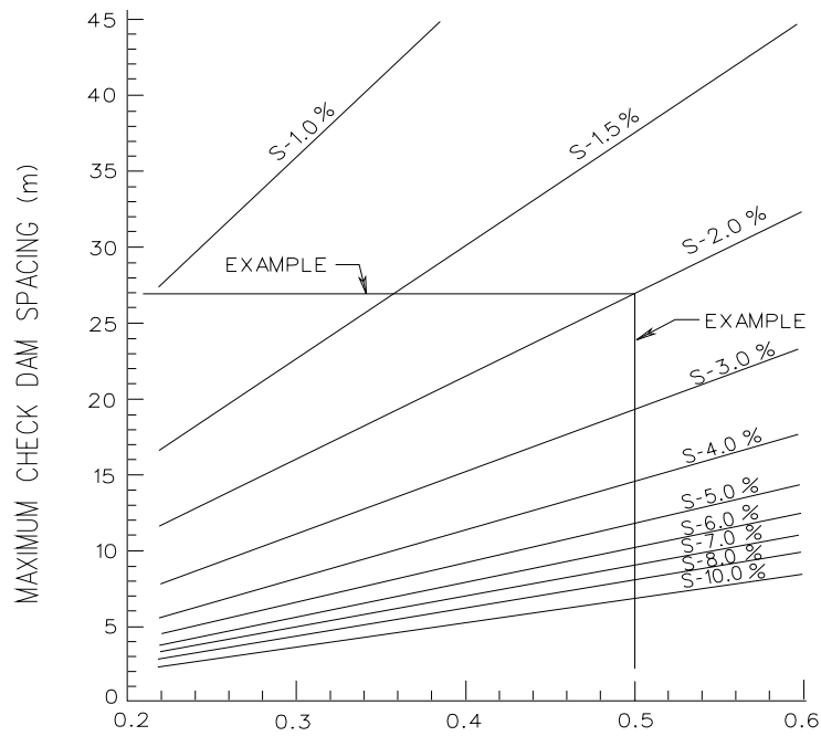
CHECK DAM HEIGHT (m) MEASURED AT BOTTOM OF SPILLWAY DESIGN OF STONE CHECK DAM SPACING ( n=0.030 , V=0.6 m/s)
