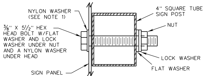
SINGLE SIGN PANEL DETAIL
