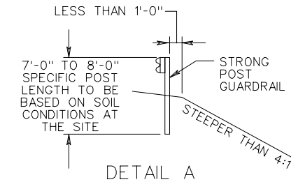
GUARDRAIL INSTALLATION SITES REQUIRING LONGER GUARDRAIL POSTS
