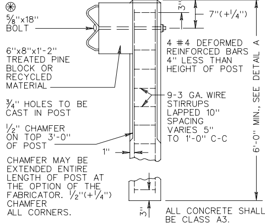
CONCRETE POST
