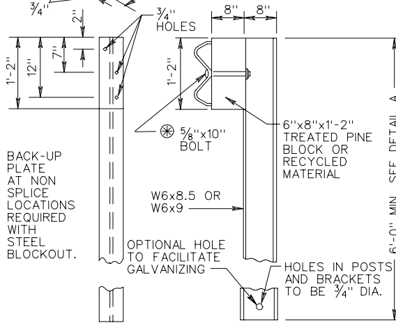
STEEL POST
