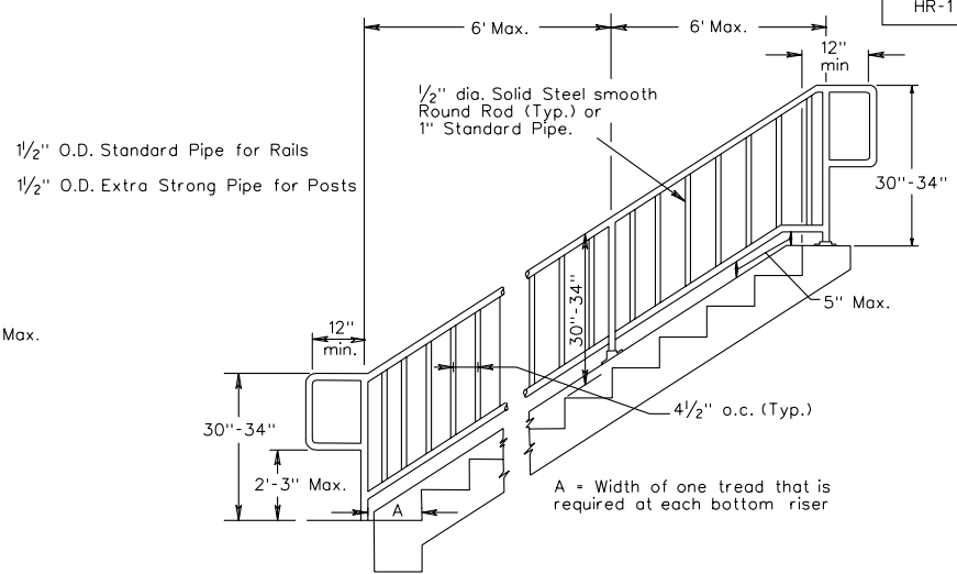
HANDRAIL INSTALLATION
