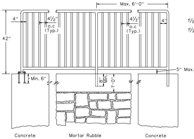
HANDRAIL (GUARD) INSTALLATION ON WALLS
