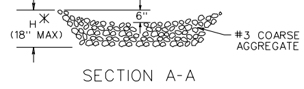
TYPICAL TREATMENT FOR DROP INLET WITH CONCRETE GUTTER
