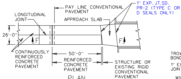
PLAN ANCHOR SLAB TYPE II (SEE NOTE 11)
