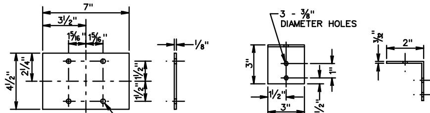
ANTI-TWIST PLATE
