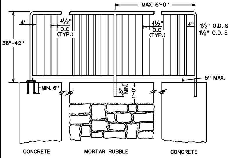
HANDRAIL (GUARD) INSTALLATION ON WALLS
