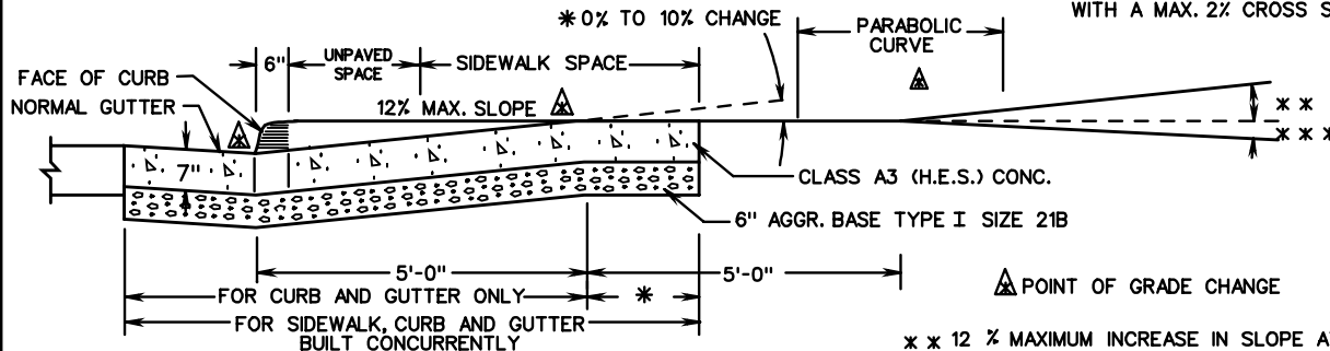
SECTION C-C
