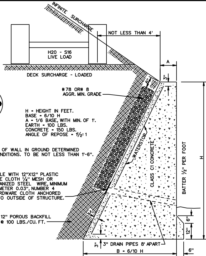
WATERSTOP DETAIL
