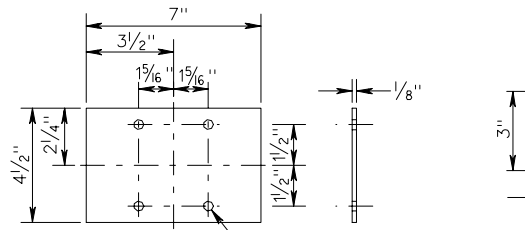
ANTI-TWIST PLATE
