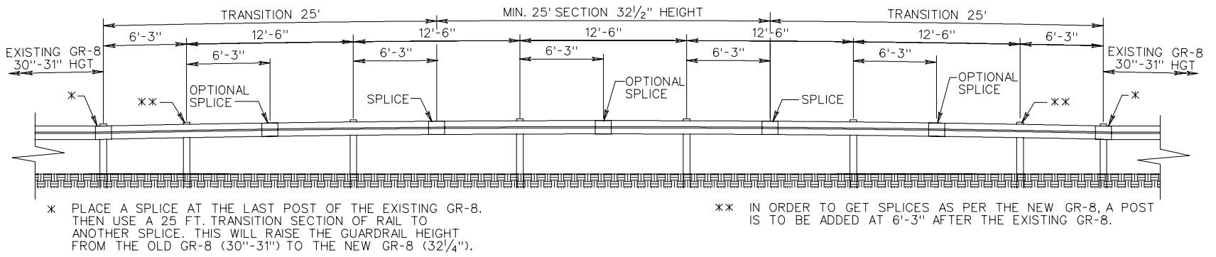
TRANSITION FROM WEAK POST (EXISTING GR-8 30"-31" HEIGHT) TO CURRENT NCHRP 350 TL-3 WEAK POST (STANDARD GR-8 32 1/4" HEIGHT)
