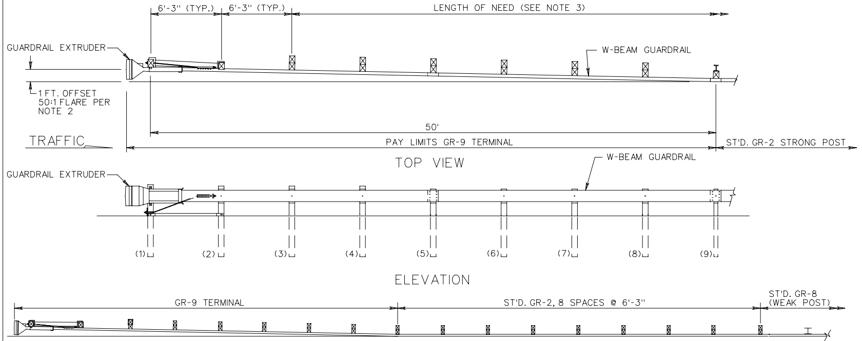
TRANSITION FROM GR-9 TERMINAL TO WEAK POST (STANDARD GR-8) GUARDRAIL
