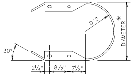
W BEAM TERMINAL CONNECTOR
