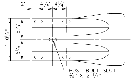
W BEAM END SECTION (FLARED)
