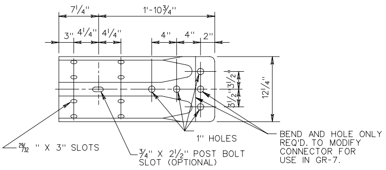
W BEAM TERMINAL CONNECTOR
