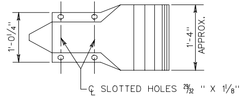
W BEAM END SECTION (BUFFER)
